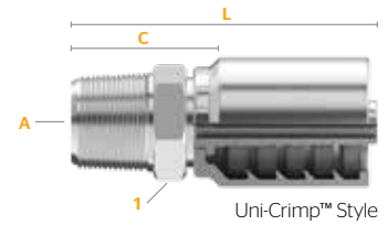
Uni-Crimp™ Style
