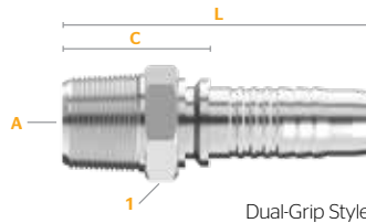
Dual-Grip Style
