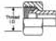
Female 24° or 60° Cone
